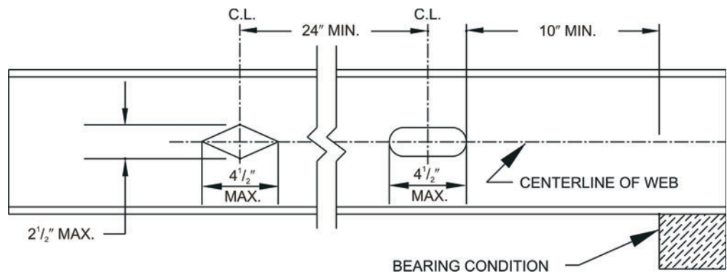
FIGURE R804.2(3) WEB HOLES
